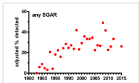
Figure 1. The percentage of barn owls ( Tyto alba ) found to be carrying residues of one or more second-generation anticoagulant in the UK 1983 to 2015. The percentage values are adjusted to take into account changes in the limits of detection provided by the different analytical methods used during the period of sampling. The data and figure is reproduced here with the kind permission of the Centre of Ecology and Hydrology [data for 2015 provided by the Campaign for Responsible Rodenticide Use].
