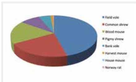
Figure 2. The percentage of different prey species in the food of barn owls in the UK. The figures are aggregate data from surveys conducted in the UK during the period 1974 to 1997 and are adjusted for mean prey weight. Note: barn owl diets are very variable and the diets of individual owls may vary considerably from that shown in the figure. Adapted from: Love, A.R., Webbon, C.E., Glue, D. and Harris, S., 2000, Changes in the food of British Barn Owls ( Tyto alba ) between 1974 and 1997, Mammal Review 30: 107-129.
